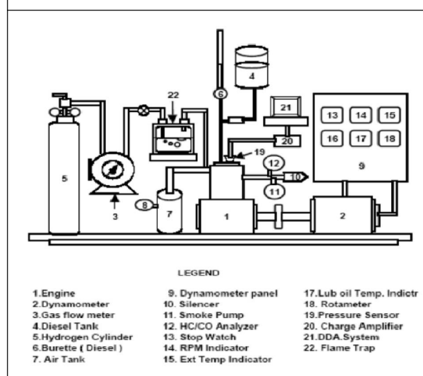
Figure 2: Sample Setup
