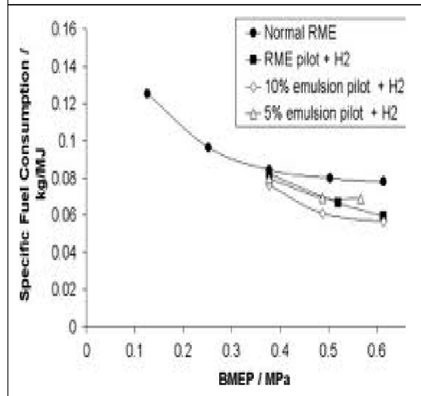
Figure 4: Reduction in Fuel Consumption With Increase in Hydrogen Addition
