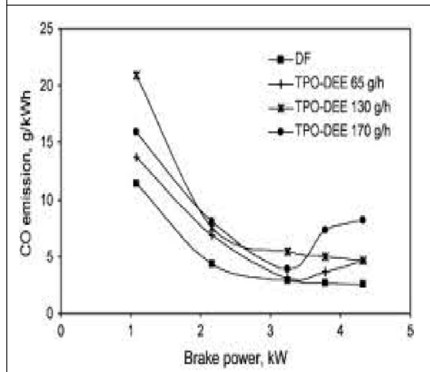
Figure 5: Effect of H 2 Addition on Jatropa Oil Combustion CO Emissions
