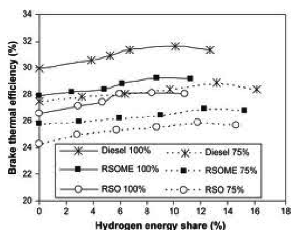
Figure 3: Variation of Thermal Efficiency With Hydrogen Mass Share
