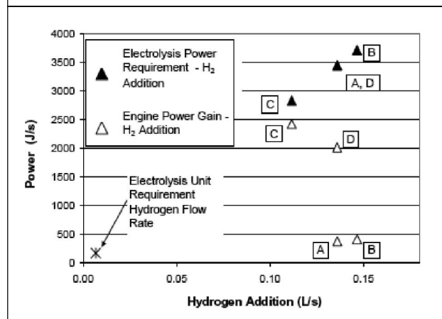
Figure 10: The Power Requirement for Electrolysis and the Power Gained from the Engine Through Hydrogen Addition
